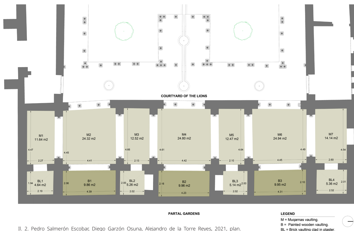
Il. 2. Pedro Salmerón Escobar, Diego Garzón Osuna, Alejandro de la Torre Reyes, 2021, plan. Descriptive plan of the Hall of the Kings with nomenclature of the ceilings of the rooms, dimensions and surfaces.
